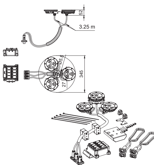
LED Modul MDD L 3D/DMX/02
