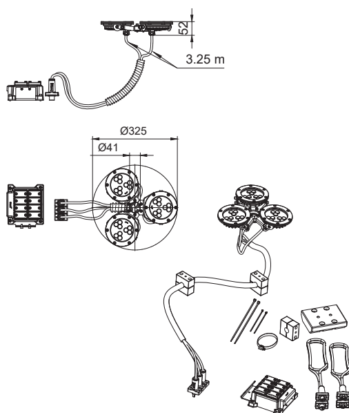
LED Modul MDD L 2D/DMX/02
